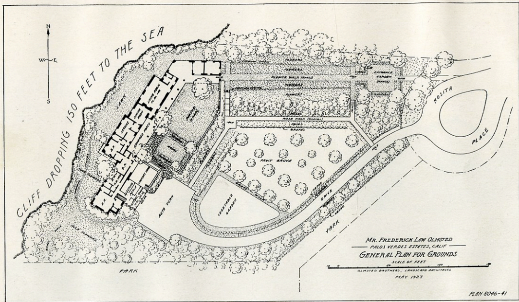
Olmsted Brothers, Landscape Architects Plan of Grounds of Mr. F. L. Olmsted at Palos Verdes
